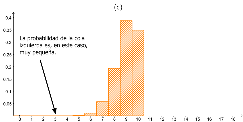
Figura 5.1: Distribución Binomiales: (a) B(10, \frac{1}{2}) . (b) B(10, \frac{1}{10}) . (c) B(10, \frac{9}{10}) .
